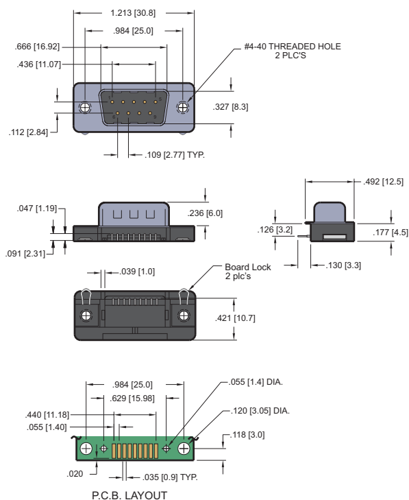
PLUG
