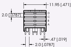
SOLDER TAIL
