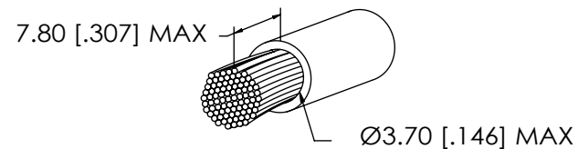
CABLE DIMENSIONS
